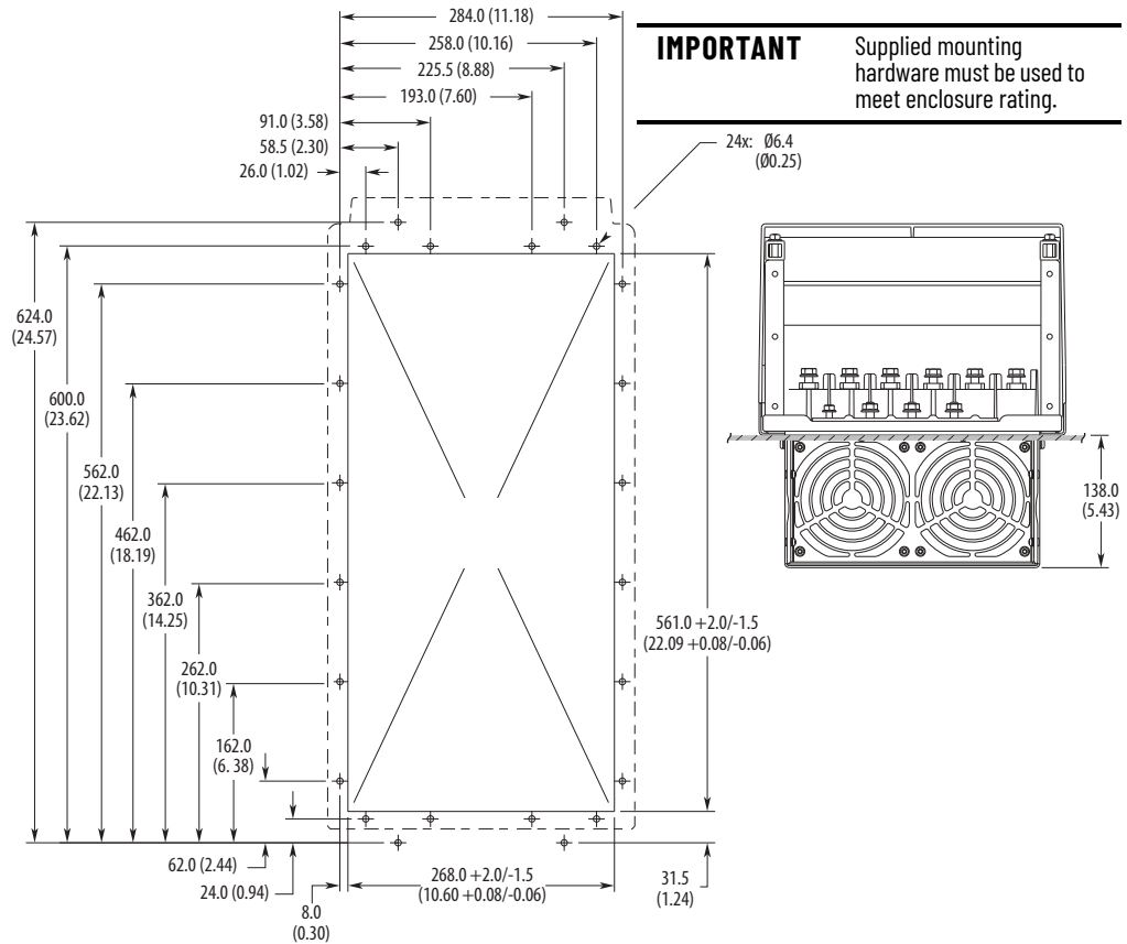
6 Flange Mount
